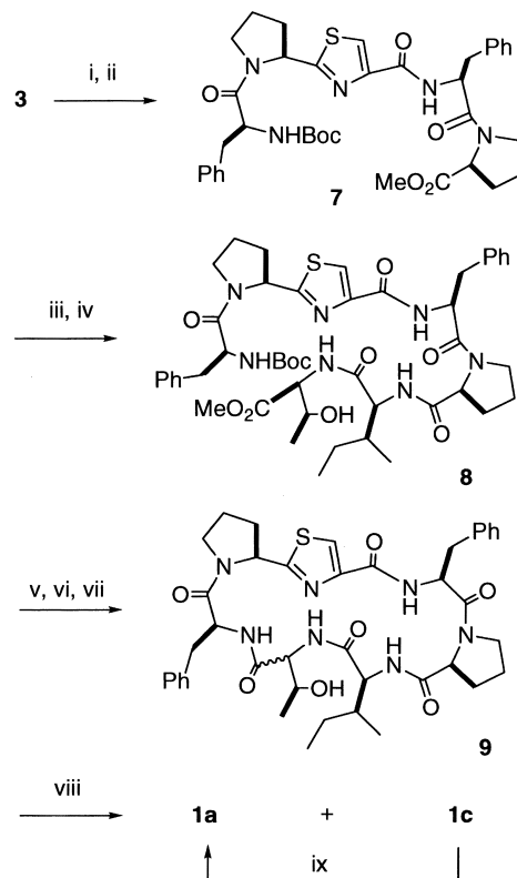
Scheme 3. Reagents: i. 1 M aq NaOH, MeOH; ii. 4 , BOP, Et 3 N, DMF (97% in 2 steps); iii. 1 M aq NaOH, MeOH; iv. 5 , BOP, Et 3 N, DMF (51% in 2 steps); v. 1 M aq NaOH, MeOH; vi. TMSOTf, CH 2 Cl 2 ; vii. DPPA, DIPEA, DMF (18% in 3 steps); viii. Deoxo-Fluor, CH 2 Cl 2 ( 1a : 12%, 1c : 46%); ix. NaOMe, MeOH (38%).
