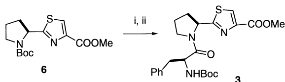
Scheme 2. Reagents: i. TFA, CH 2 Cl 2 , 0 °C; ii. Boc-L-Phe-OH, BOP, Et 3 N, DMF (78% in 2 steps).
