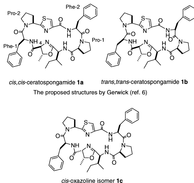
Fig. 1. Chemical Structures of ceratospongamides.
